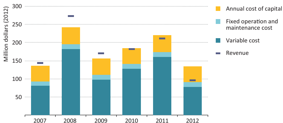
Figure 3.16 ▶ Allocation of revenues for a high-efficiency CCGT in a competitive European electricity market, 2007-2012
