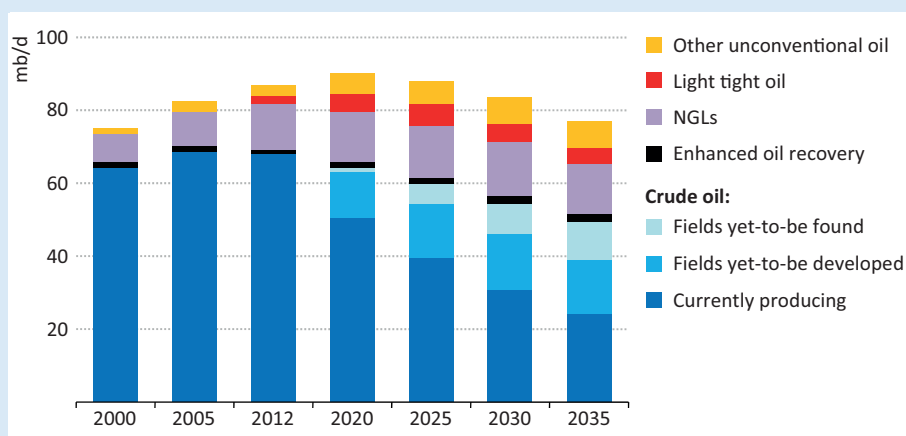
Figure 2.24 ▶ World oil production by type in the 450 Scenario
