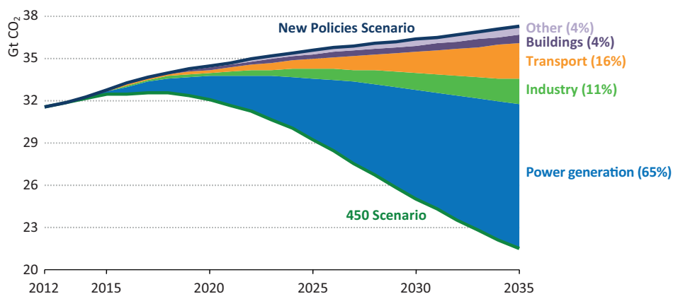
Figure 1.12 ▶ World energy-related CO 2 emissions by scenario
