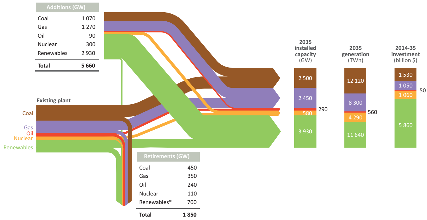
Figure 3.5 ▶ Power generation global capacity flows and investment, 2014-2035
