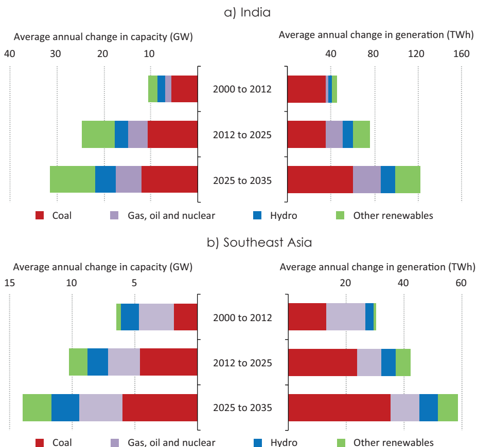
Figure 3.21 ▶ India and Southeast Asia average annual change in capacity and electricity generation in the New Policies Scenario
