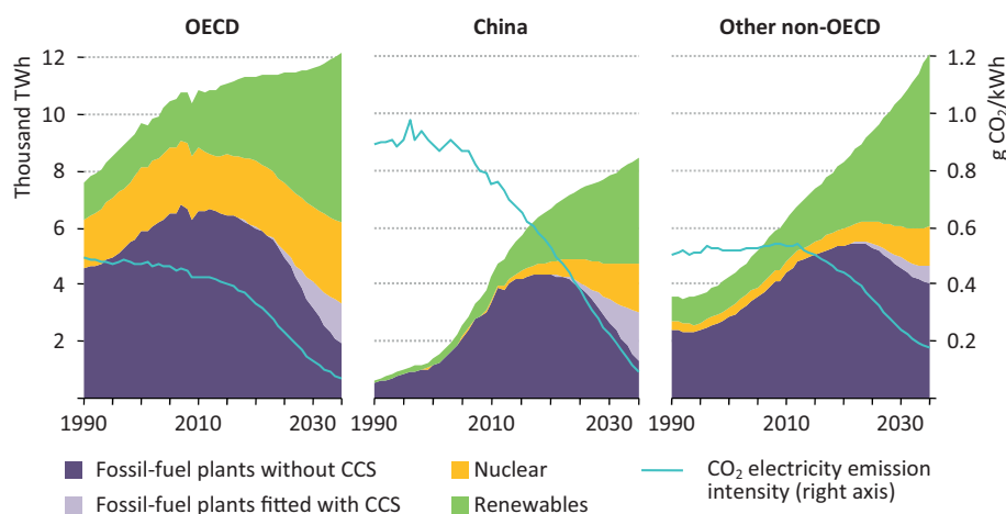
Figure 3.22 ▷ Electricity generation by technology and CO 2 intensity in the 450 Scenario
