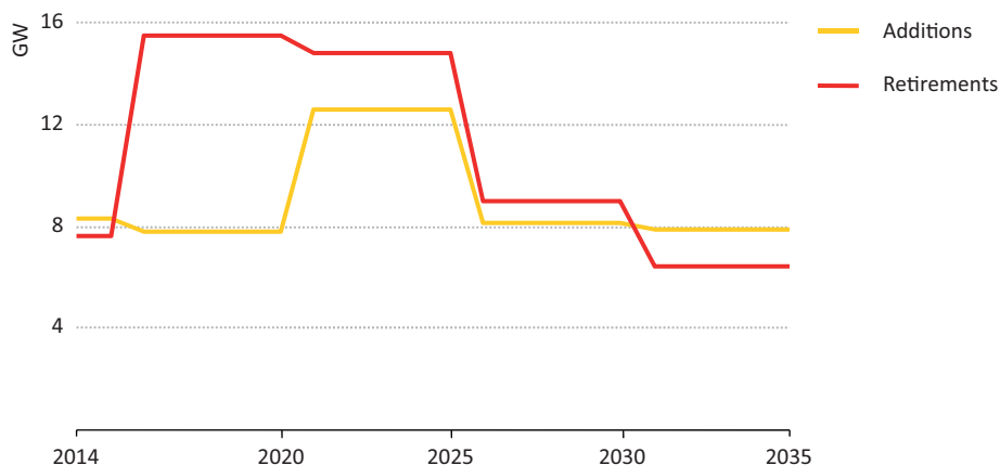
Figure 3.17 ▶ Average retirements and capacity additions of thermal plants in the European Union in the New Policies Scenario
