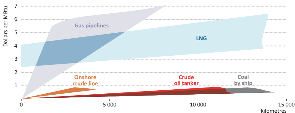
Figure 2.15 ▶ Indicative comparison of fossil fuel transportation costs
