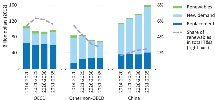
Figure 3.10 ▶ Average annual investment in T&D infrastructure in the New Policies Scenario
