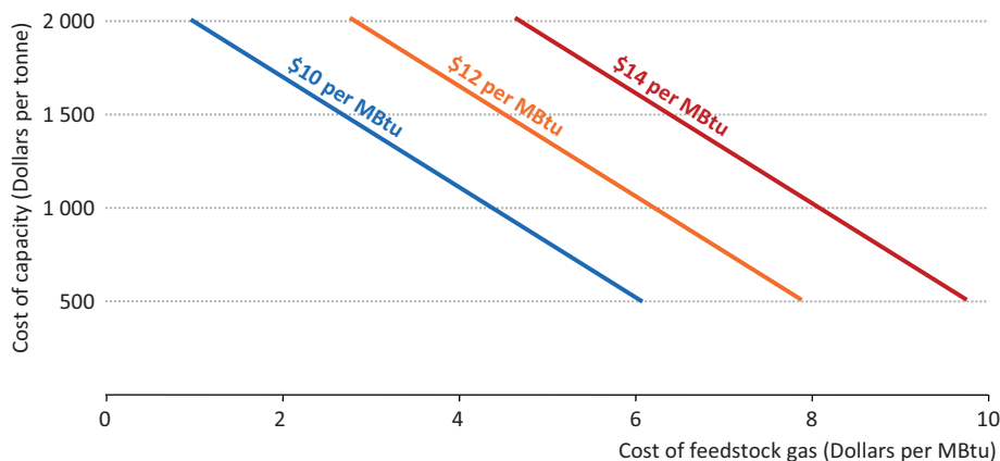
Figure 2.17 ▶ Indicative trade-off between the costs of new LNG capacity and of gas feedstock for a range of delivered prices
