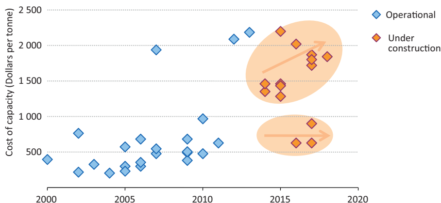
Figure 2.16 ▶ Diverging trends in the evolution of capacity costs for global LNG liquefaction projects
