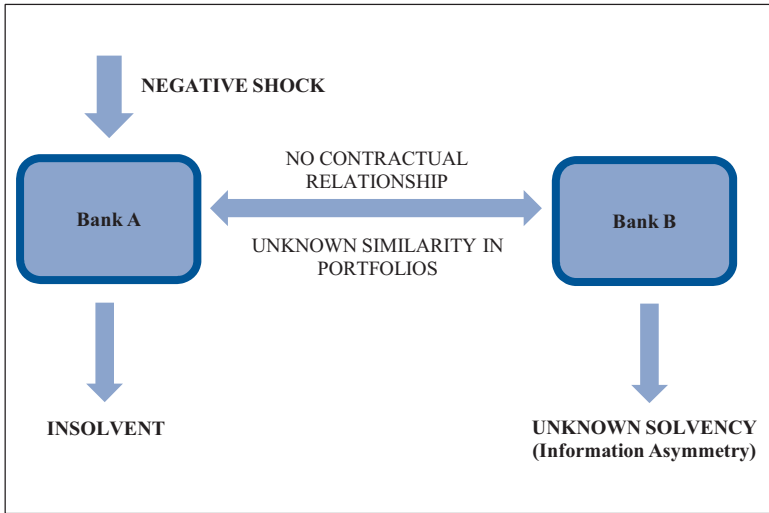
Figure 6-4 Confidence Contagion
