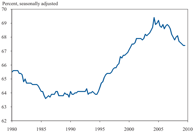
Figure 4-6 Homeownership Rate
