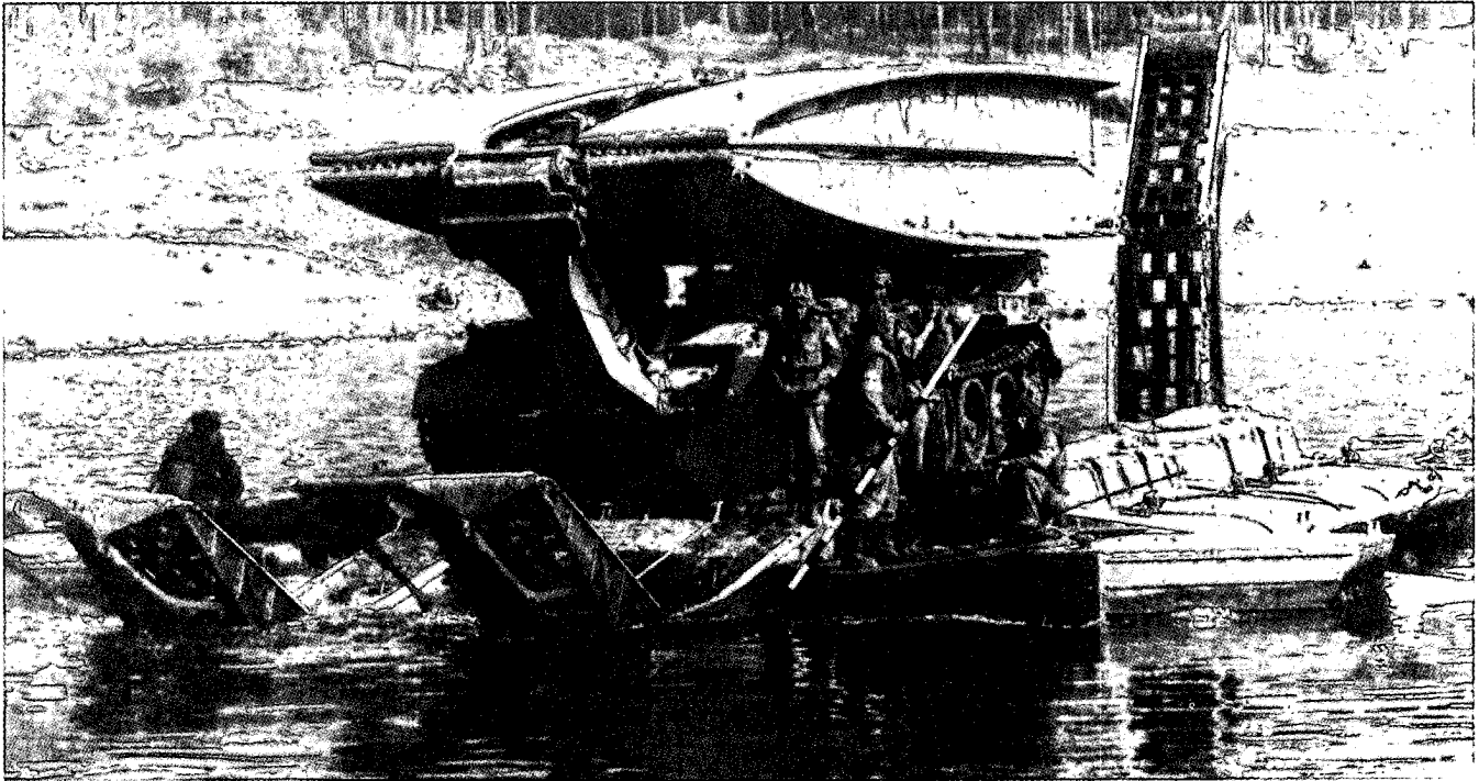
In the 1980s, Soviet ground forces have fielded a new bridge/ferry system to augment their river-crossing capability; here, a heavy amphibious ferry transports a tank-mounted scissors bridge.
