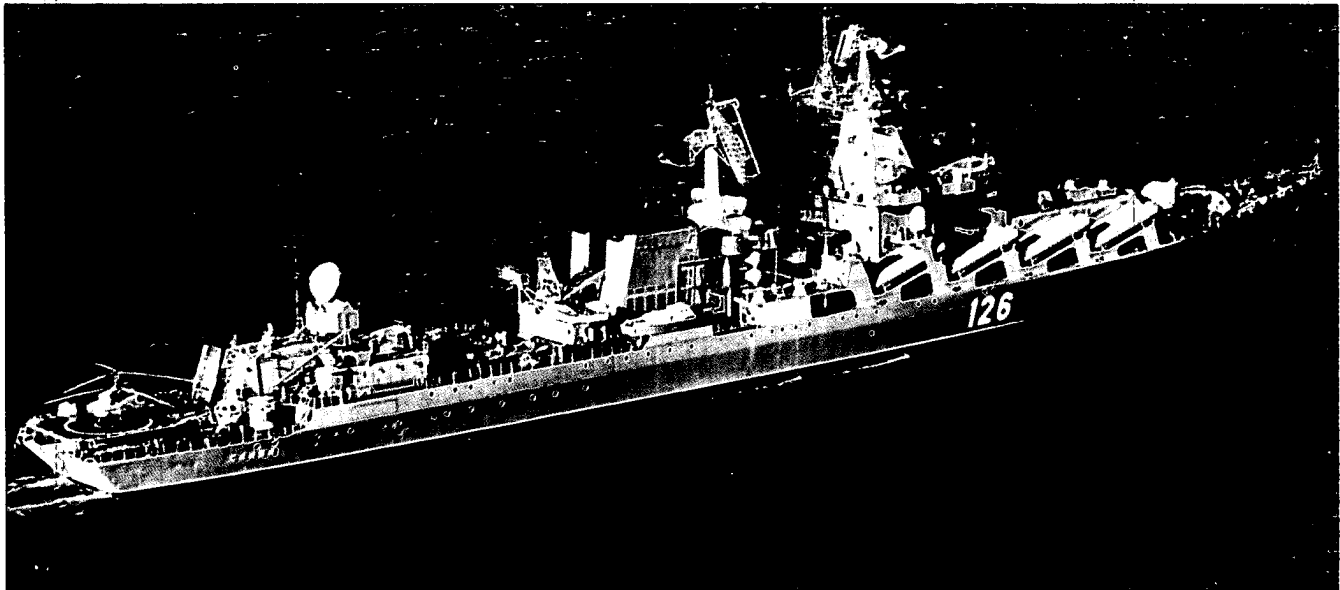
The SLAVA-Class guided-missile cruiser carries sixteen, 550-kilometer antiship cruise missiles as well as air- and point-defense missiles and a 130-mm twin-barrel gun.
