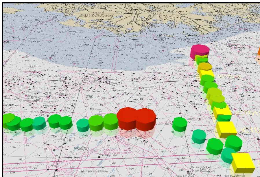
Figure 28. Westernmost Anomaly.
