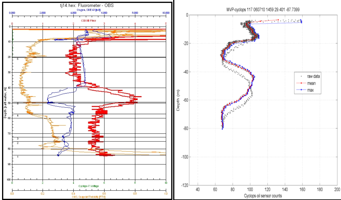
Figure 23. CTD cast in comparison area.
